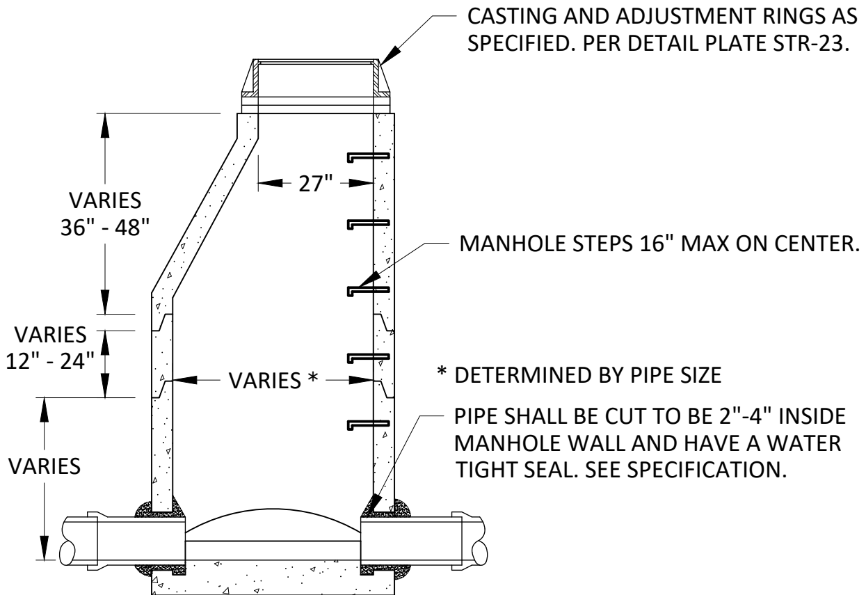
SECTION
