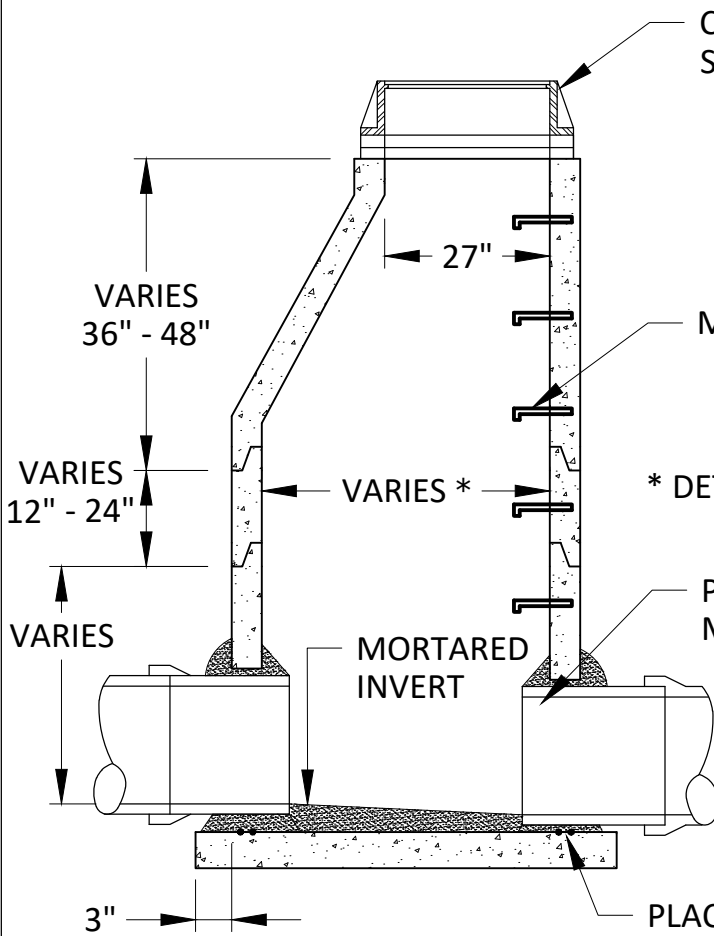
SECTION
